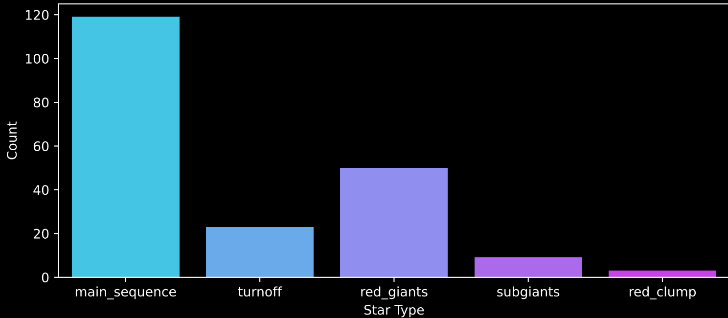
APOGEE DR17 Field: [210+75] Count plot of Star Type
