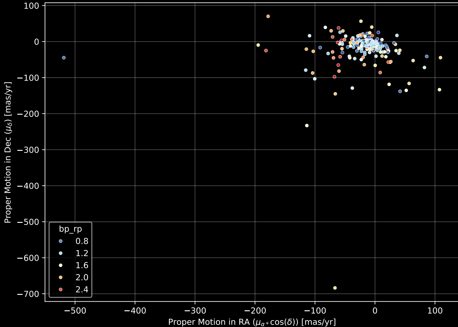
APOGEE DR17 Field: [210+75] Proper Motion Diagram (n= 204)
