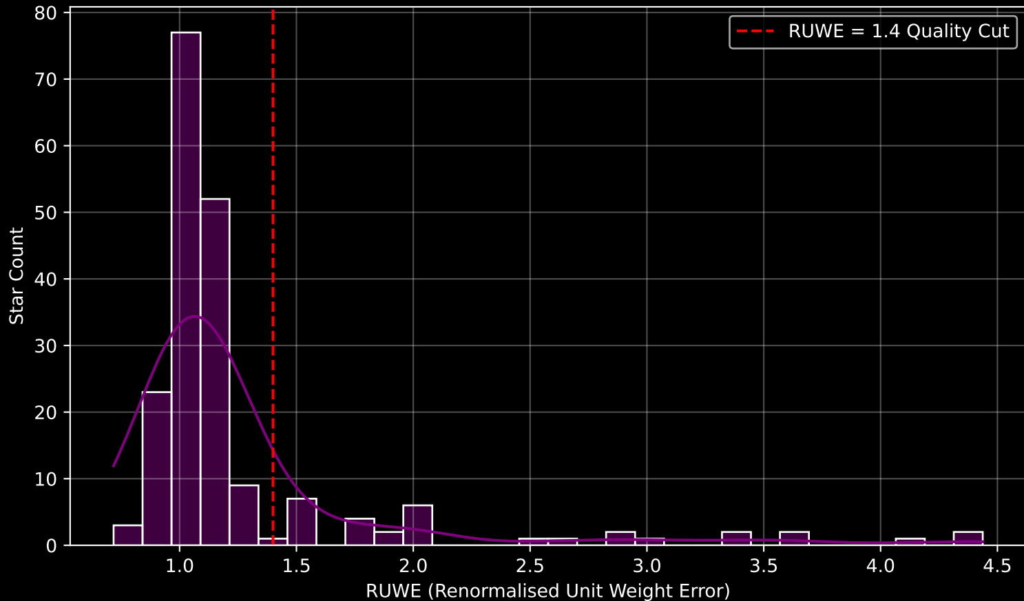
GAPOGEE DR17 Field [210+75] RUWE Distribution (n= 196)
