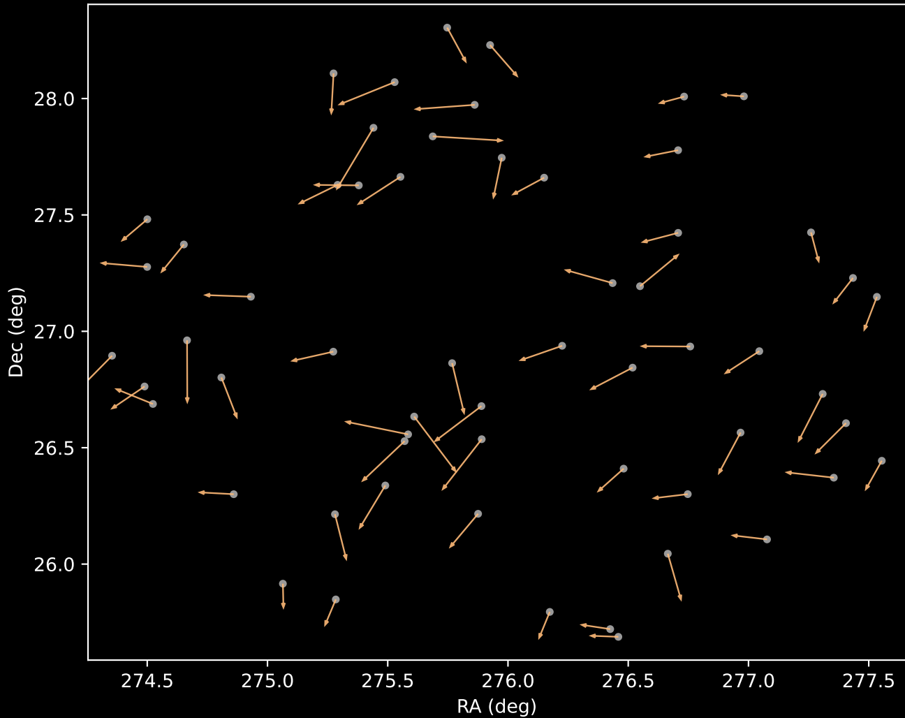
APOGEE DR17 Cluster 3 Proper Motion Vectors (n=59)
