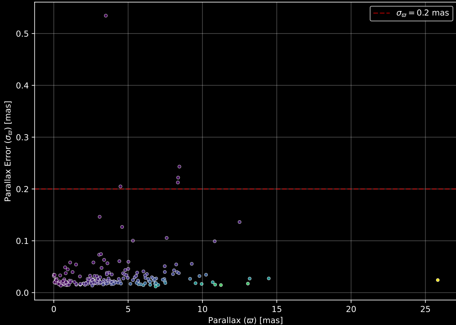
APOGEE DR17 Field: [210+75] Parallax Quality (n= 204)
