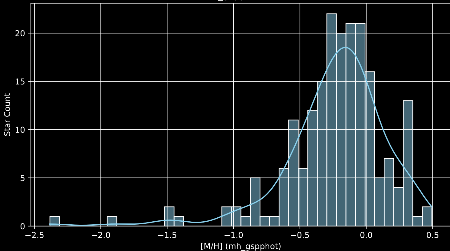
APOGEE DR17 Field: [210+75 [M/H] (mh_gspphot) (n= 199)
